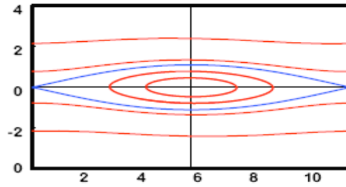
Figure 1: Phase-space portrait of a typical BGK equilibrium.
